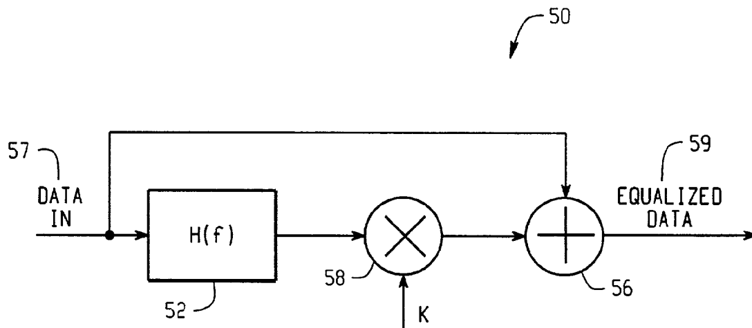
Fig. 4 RELATED ART
